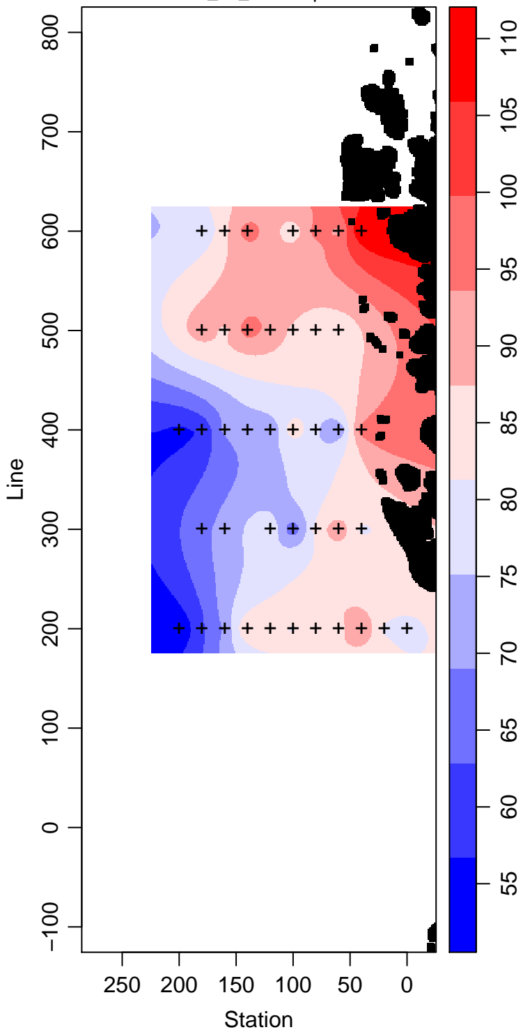
PD95-01_90_Silicate \mu\text{ mol L}^{-1}
