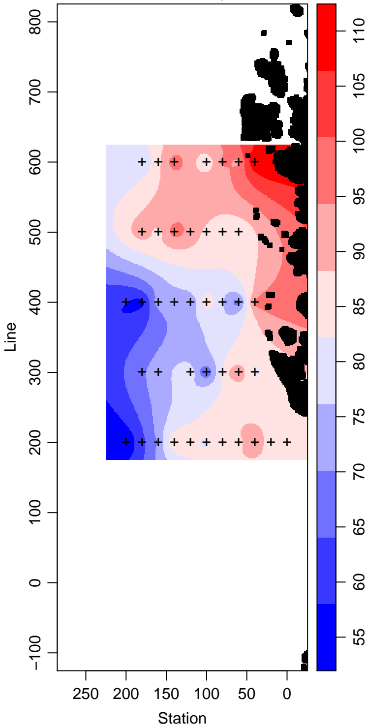
PD95-01_95_Silicate \mu\text{ mol L}^{-1}
