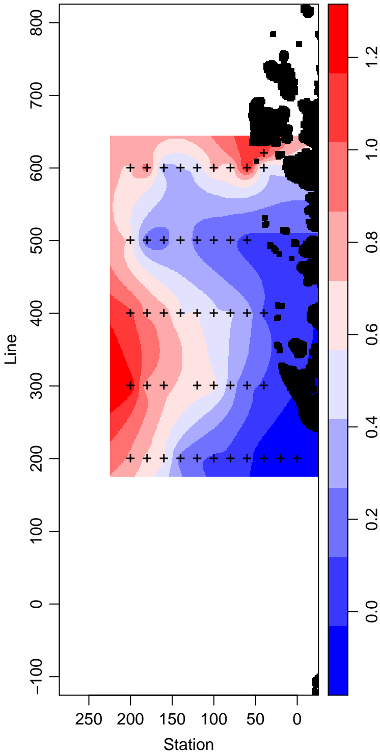
PD95-01_5_Temperature ° Celsius
