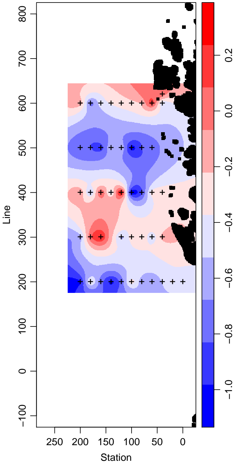
PD95-01_60_Temperature ° Celsius
