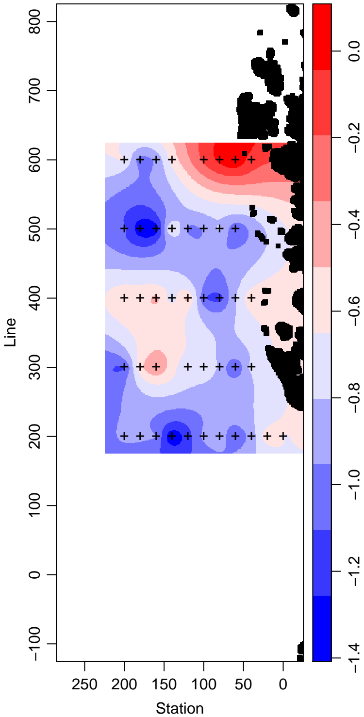
PD95-01_75_Temperature ° Celsius
