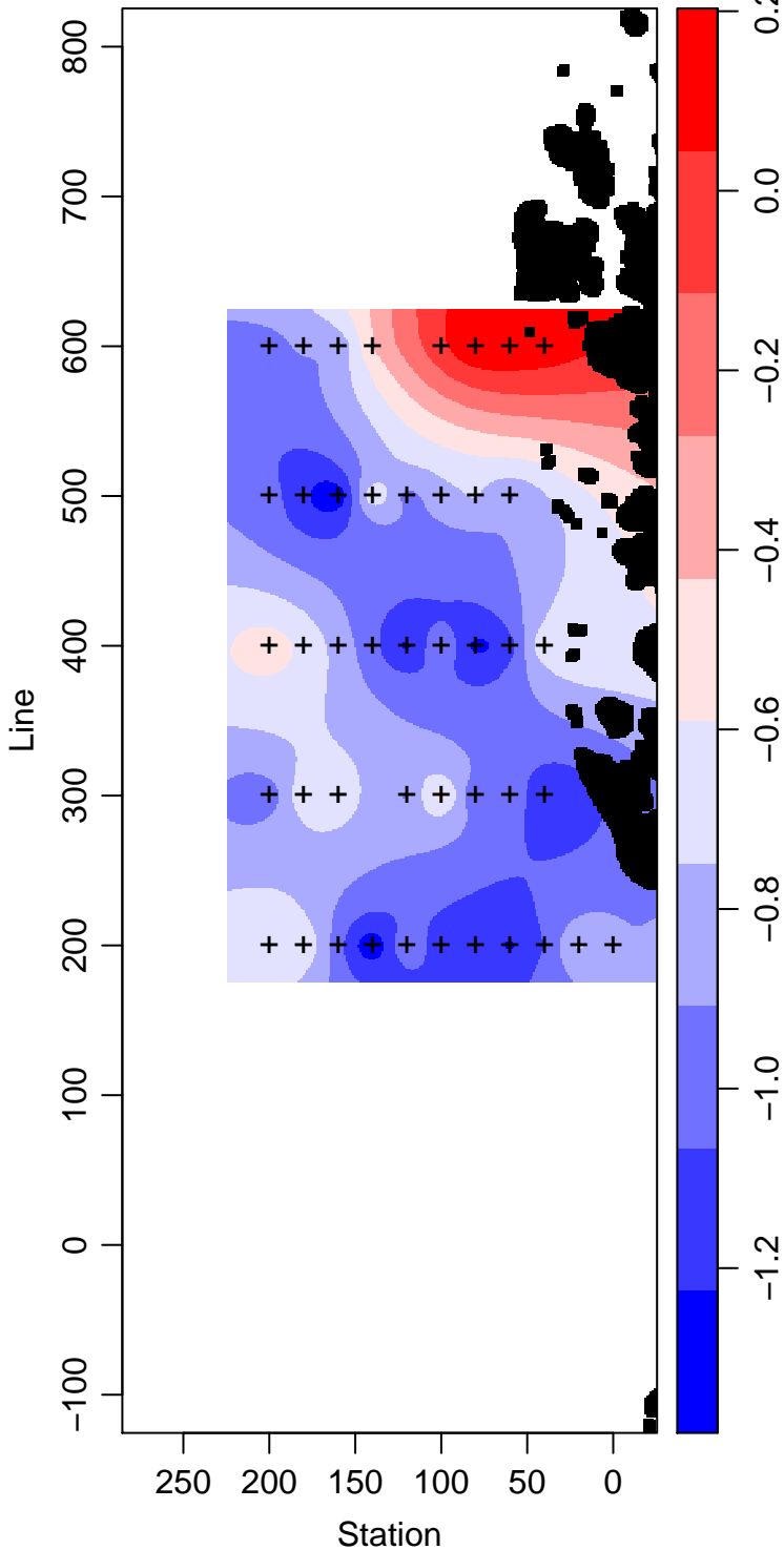
PD95-01_90_Temperature ° Celsius
