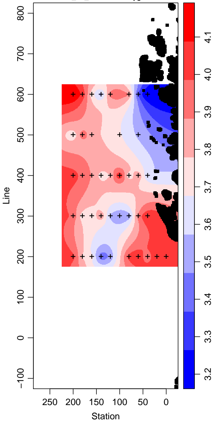
PD96-01_45_Dissolved.Oxygen ml L -1
