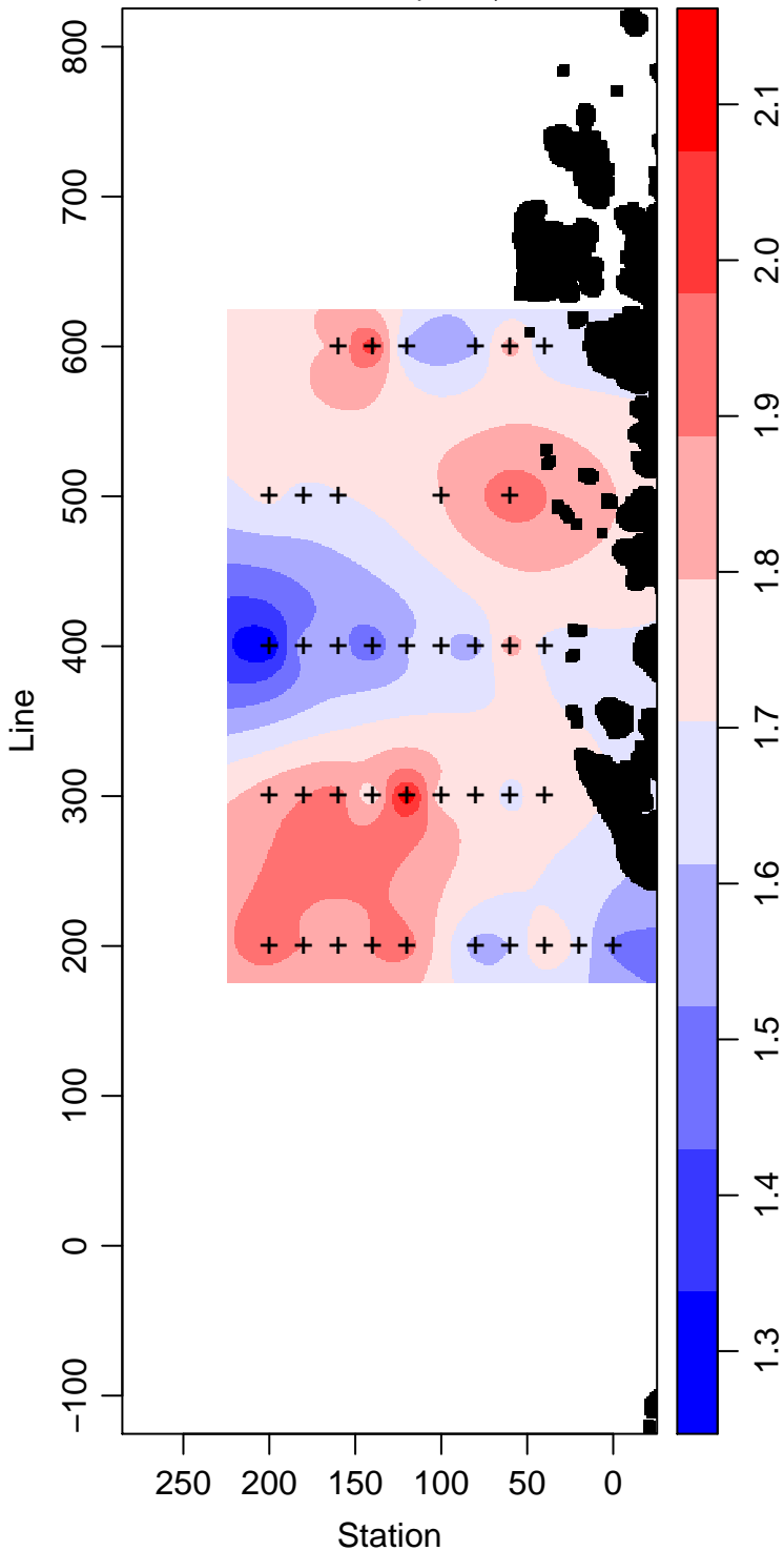
PD96-01_35_Phosphate \mu\text{ mol L}^{-1}
