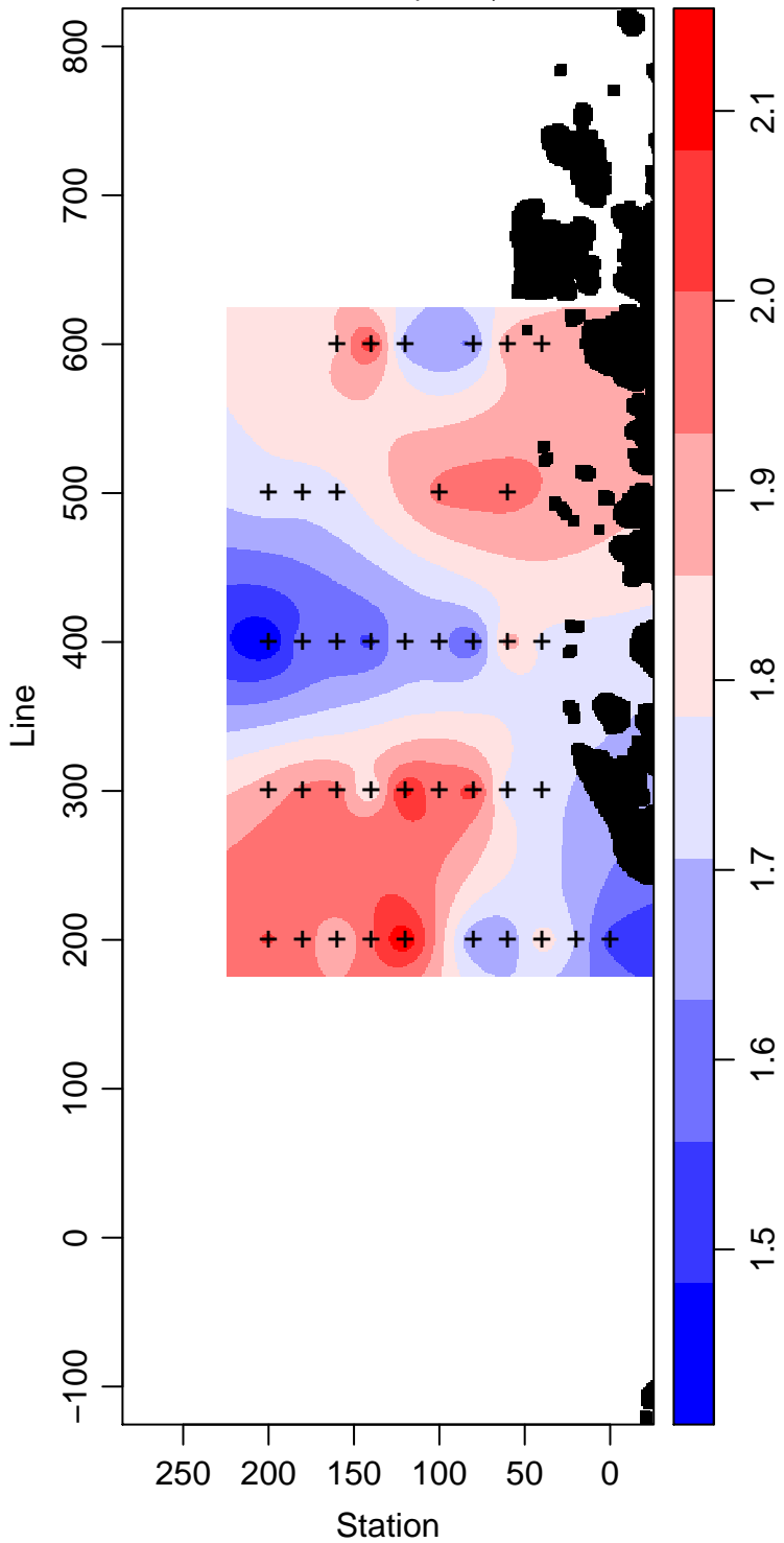
PD96-01_40_Phosphate \mu\text{ mol L}^{-1}
