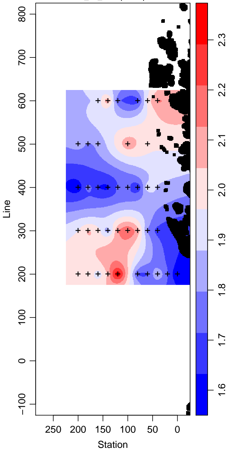
PD96-01_45_Phosphate \mu\text{ mol L}^{-1}
