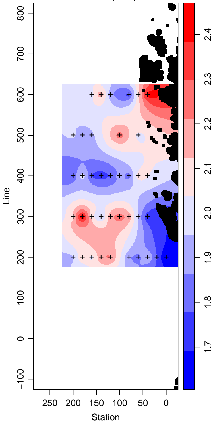
PD96-01_55_Phosphate \mu\text{ mol L}^{-1}
