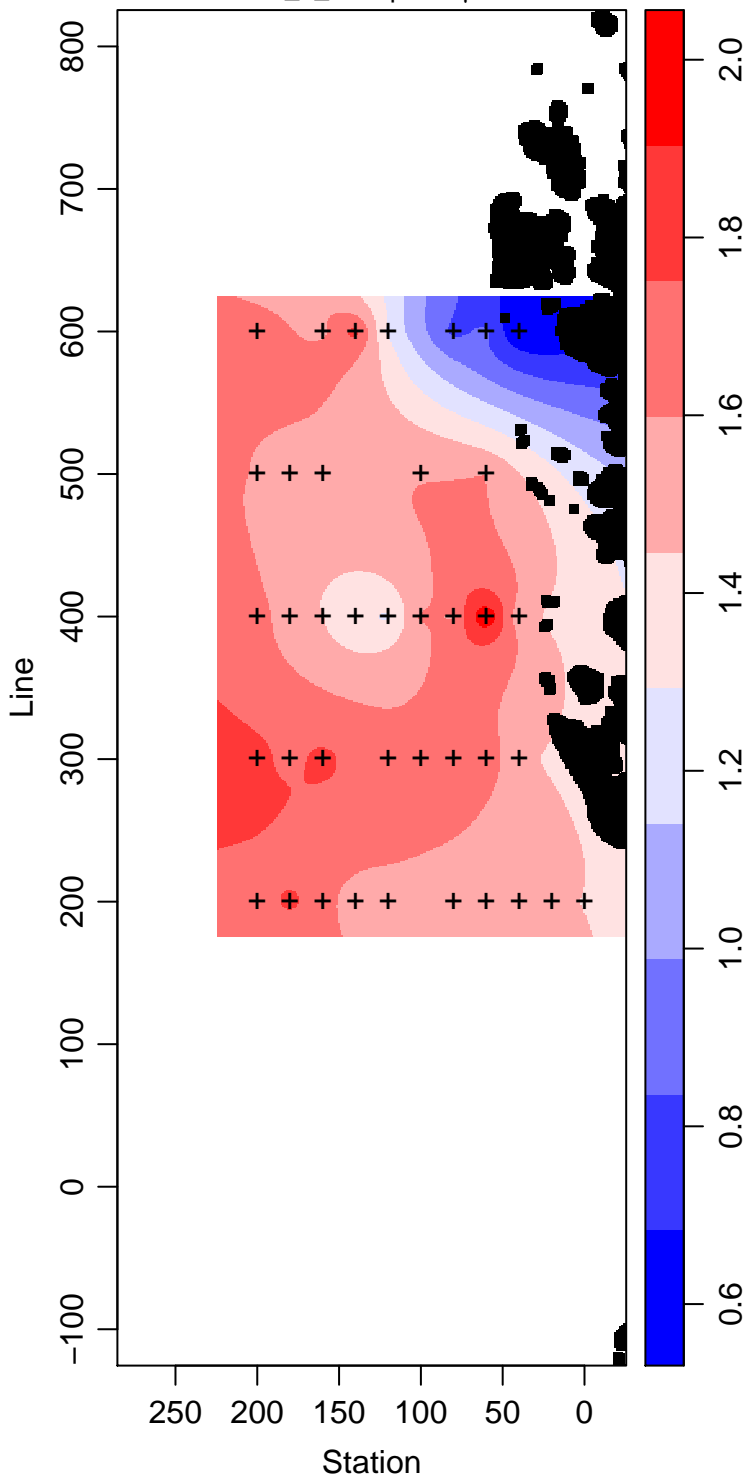
PD96-01_5_Phosphate \mu\text{ mol L}^{-1}
