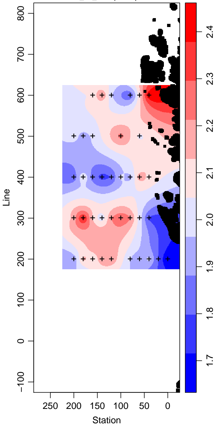
PD96-01_60_Phosphate \mu\text{ mol L}^{-1}
