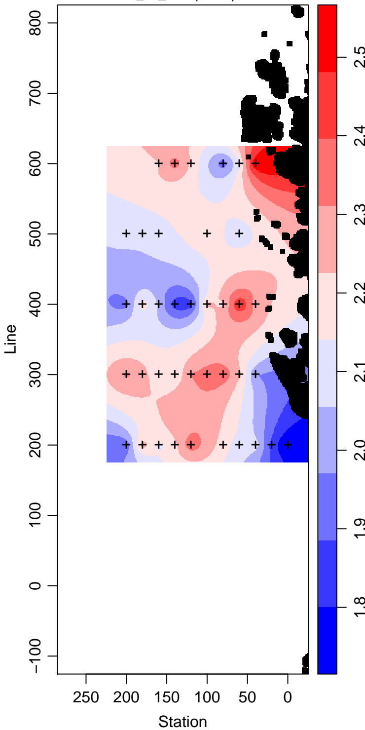
PD96-01_75_Phosphate \mu\text{ mol L}^{-1}
