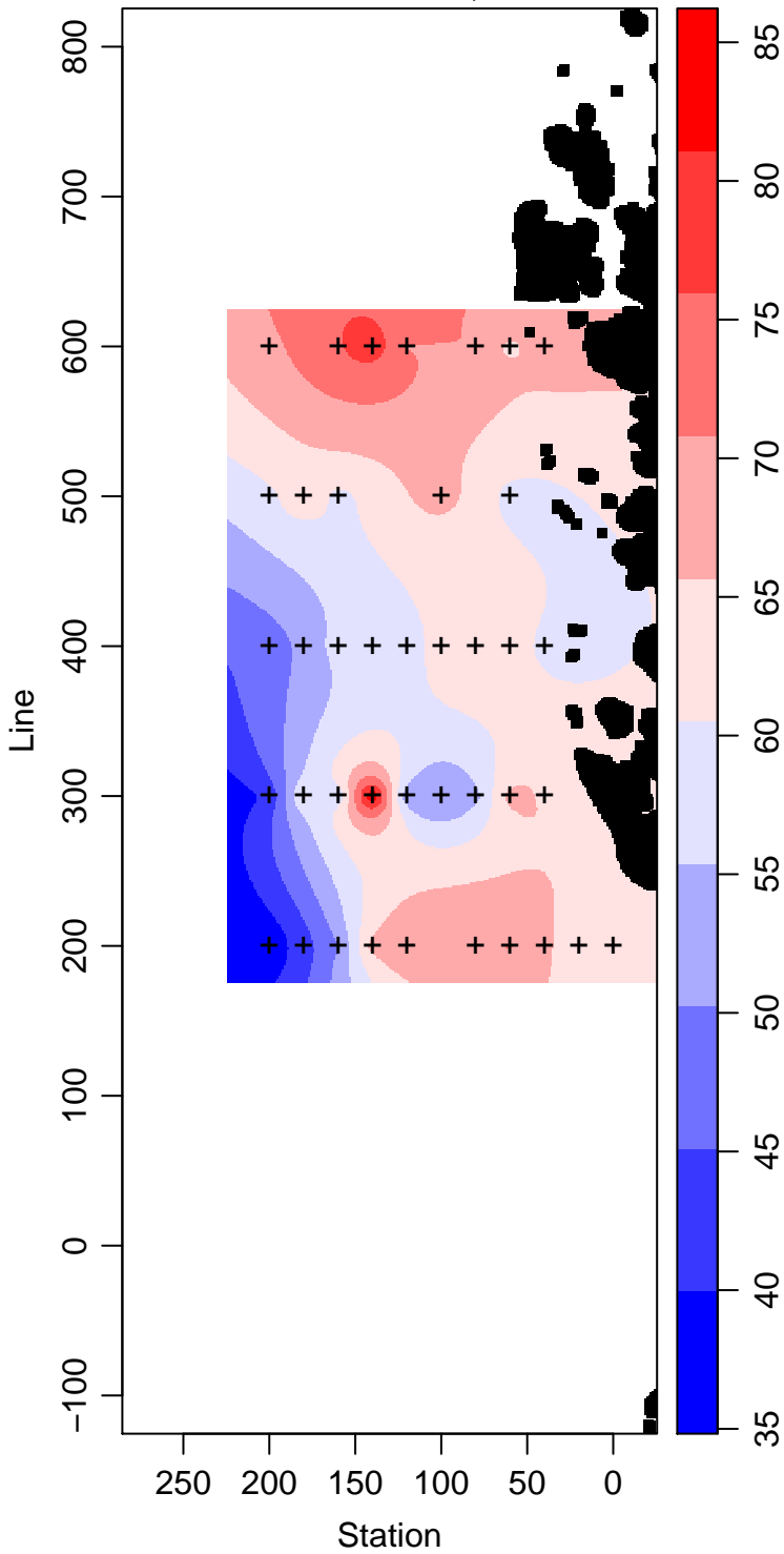
PD96-01_15_Silicate \mu\text{ mol L}^{-1}
