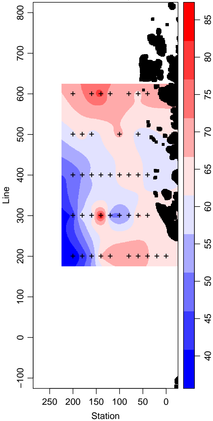
PD96-01_20_Silicate \mu\text{ mol L}^{-1}
