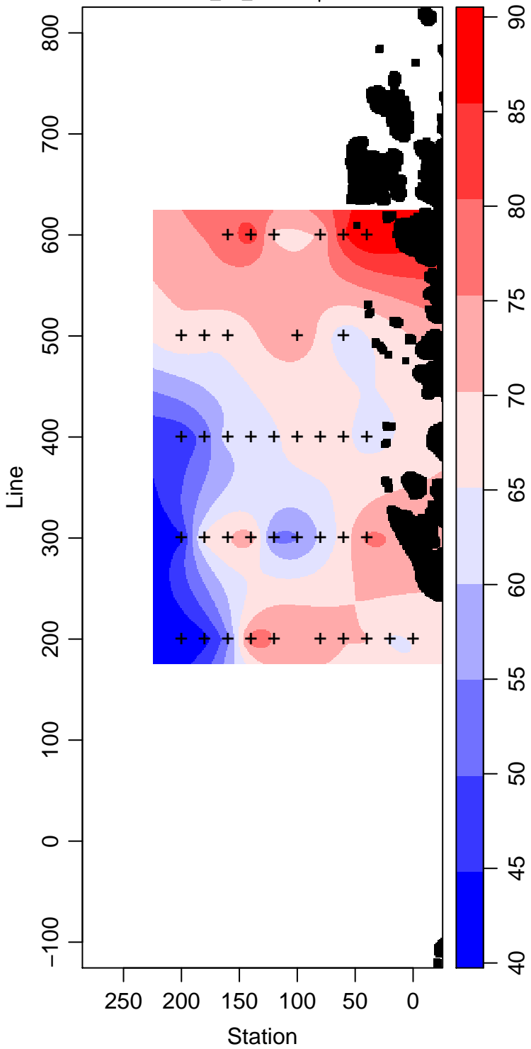
PD96-01_40_Silicate \mu\text{ mol L}^{-1}
