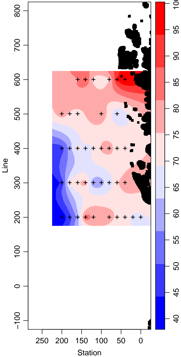
PD96-01_55_Silicate \mu\text{ mol L}^{-1}
