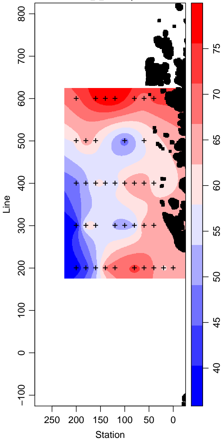
PD96-01_5_Silicate \mu\text{ mol L}^{-1}
