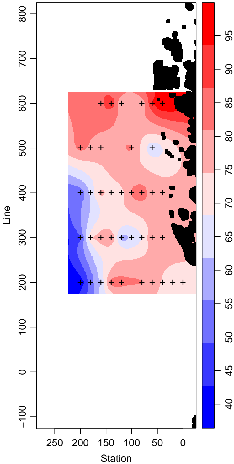
PD96-01_65_Silicate \mu\text{ mol L}^{-1}
