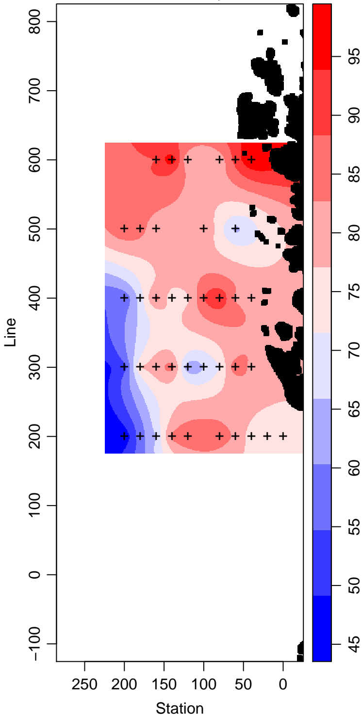
PD96-01_80_Silicate \mu\text{ mol L}^{-1}
