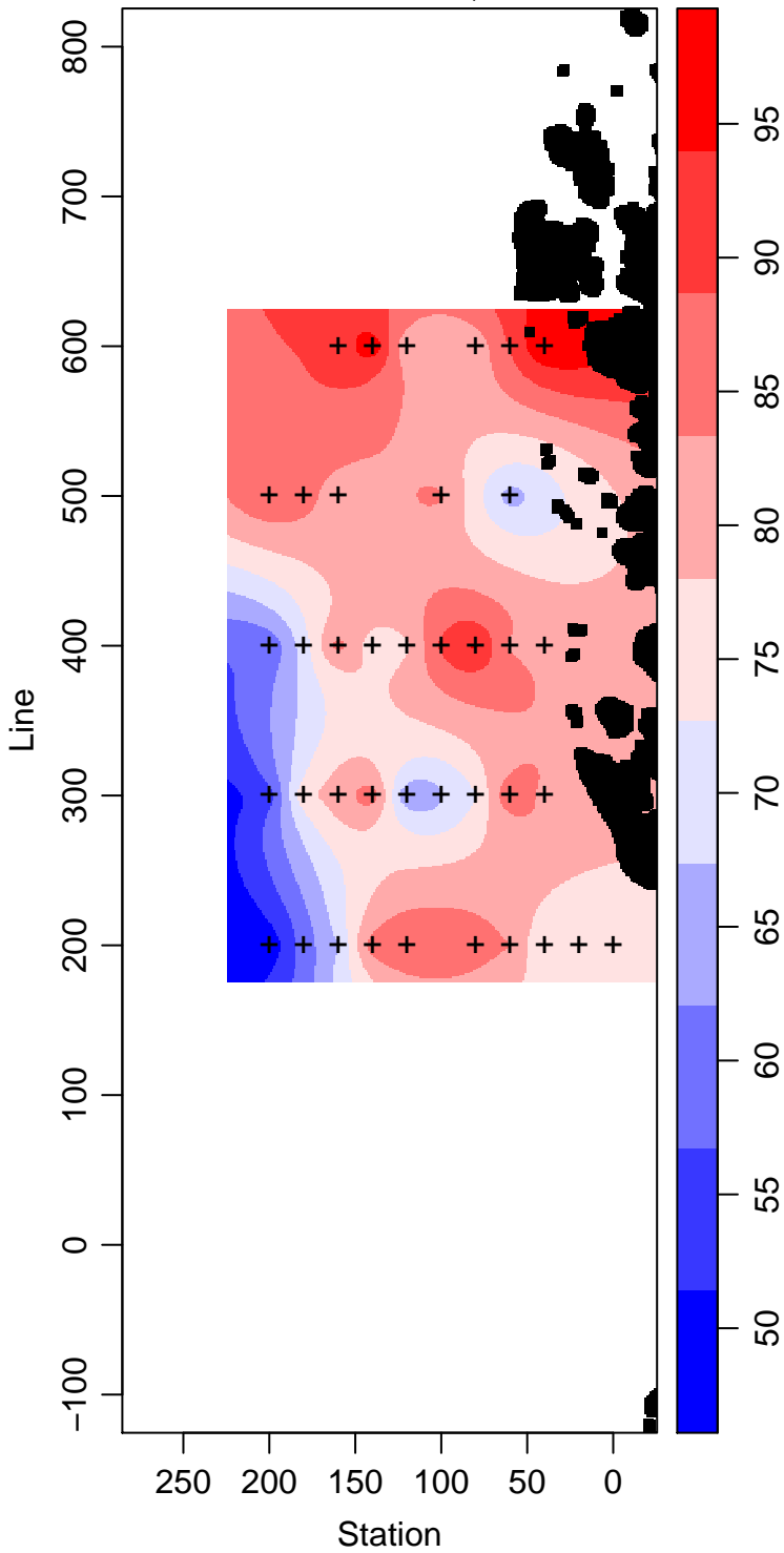
PD96-01_85_Silicate \mu\text{ mol L}^{-1}
