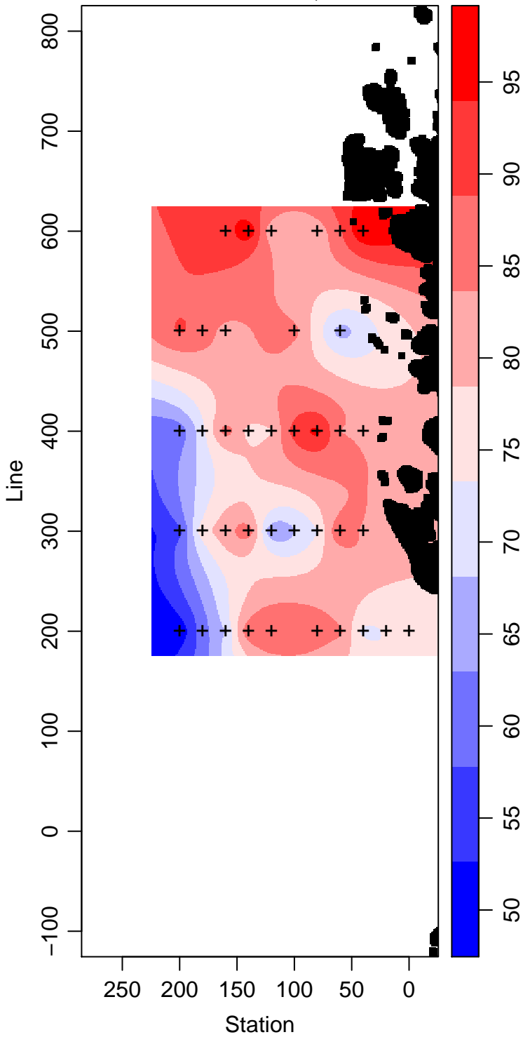
PD96-01_90_Silicate \mu\text{ mol L}^{-1}
