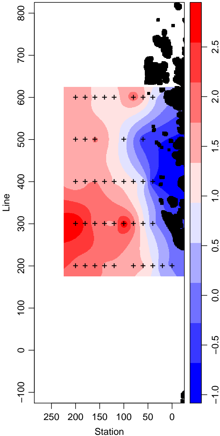
PD96-01_1_Temperature ° Celsius
