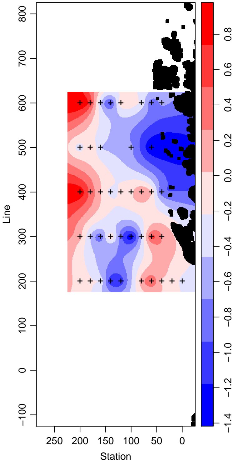
PD96-01_45_Temperature ° Celsius
