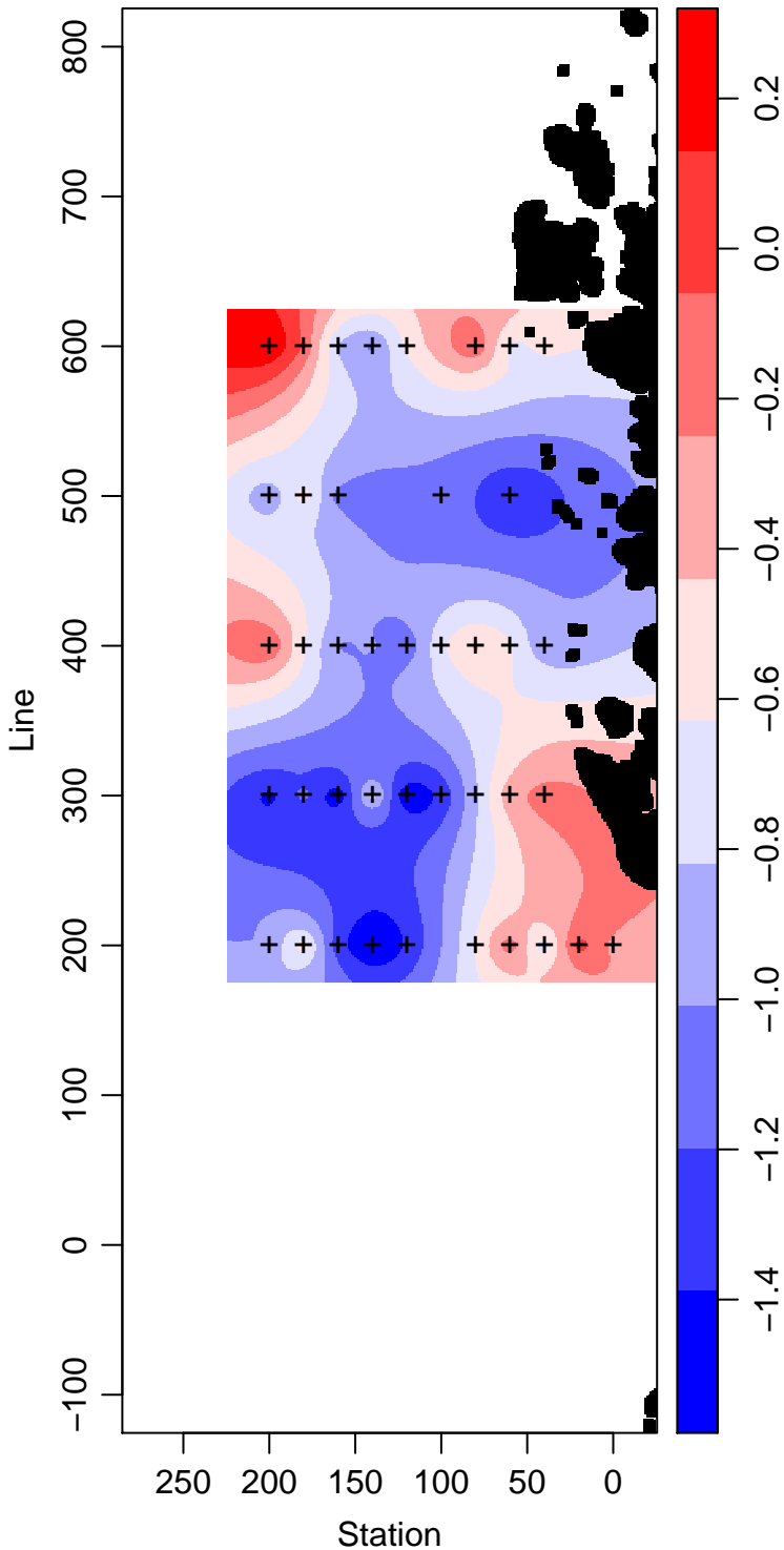
PD96-01_60_Temperature ° Celsius
