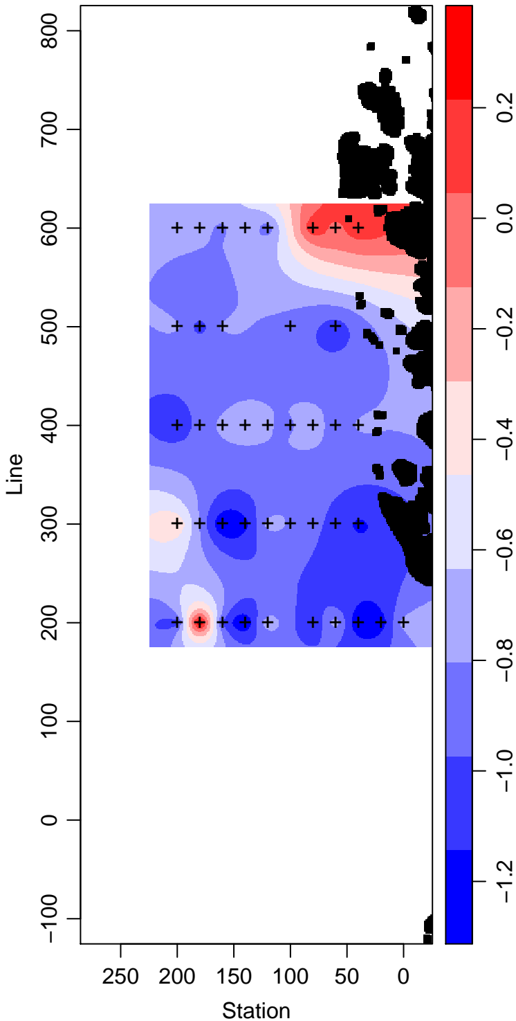
PD96-01_95_Temperature ° Celsius
